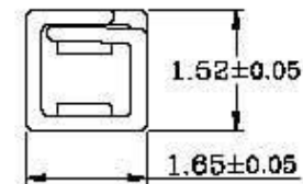
Section C-C
