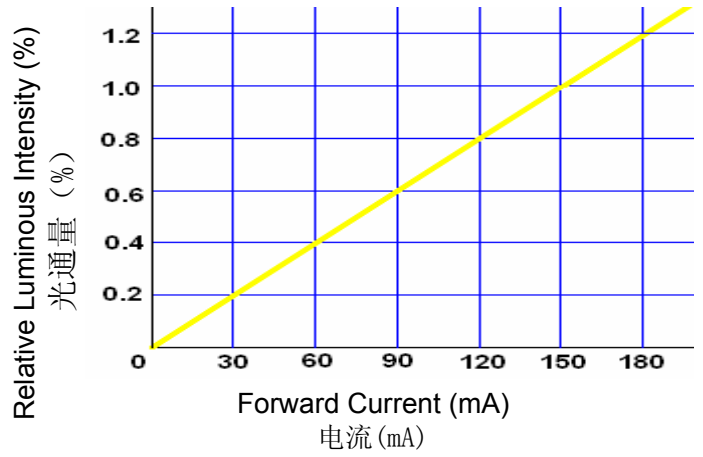
Forward Current vs Relative Luminous Intensity 电流和光通量的关系
