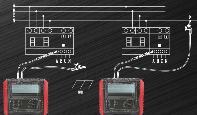
3-phase 4-wire RCD test
