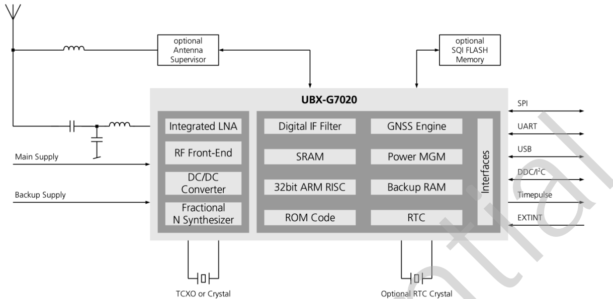
Figure 1: u-blox 7 block diagram
