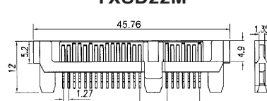
7+15P SERIAL ATA MALE DIP TYPE YXSD22M
