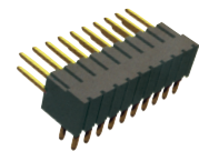
PIN HEADER DUAL ROWS (RIGHT ANGLE) YXRxx
