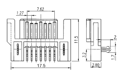
7P SERIAL ATA MALE SMD TYPE YXSD07M
