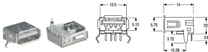
Y99000 USB/A TYPE SOCKET
