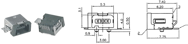
Y98900 4P MINI USB/A TYPE SOCKET (SMD TYPE)
