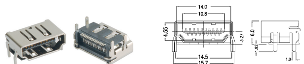
Y99065 19P HDMI SOCKET (SMD TYPE)
