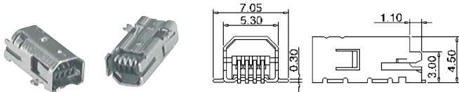
Y98902 4P MINI USB/B TYPE SOCKET (SMD TYPE)
