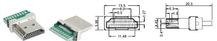
Y99061 19P HDMI PLUG
