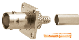
M55760 BNC FEMALE CHASSIS CRIMP TYPE (RG58U/59U)
