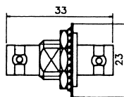
M55775 BNC FEMALE BULKHEAD CRIMP TYPE (RG174U) M55775T TEFLON INSULATION
