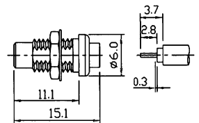
M52096 SMC FEMALE BULKHEAD SOLDER TYPE FOR SEMI-RIGID CABLE (RG402U/405U) (GOLD PLATED)
