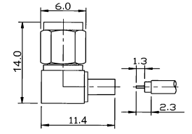
M52092 RIGHT ANGLE SMC MALE SOLDER TYPE FOR SEMI-RIGID CABLE (RG402U/405U) (GOLD PLATED)
