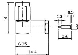
M52016 RIGHT ANGLE SMC MALE CLAMP TYPE (RG174U/178U) (GOLD PLATED)
