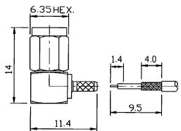
M52004 RIGHT ANGLE SMC MALE CRIMP TYPE (RG174U/178U) (GOLD PLATED)
