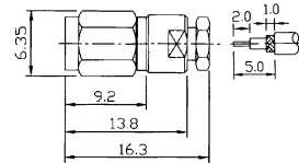
M52090 SMC MALE SOLDER TYPE FOR SEMI-RIGID CABLE (RG402U/405U) (GOLD PLATED)
