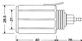
K3216 AUTO PLUG TO AUTO DOUBLE JACK LIGHT RING & BATTERY CHECKER W/FUSE/10A
