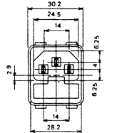
K241530 PANEL MOUNT MULTI AC SOCKET TERMINAL 4.8mm
