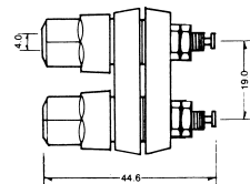
K2101 BINDING POST (GOLD PLATED)
