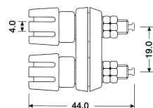
K2104 DOUBLE BINDING POST (GOLD PLATED)
