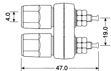
K2103 (GOLD PLATED)
