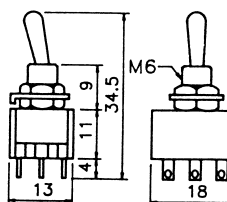
B068EW 6P MINIATURE TOGGLE SWITCH (DPDT) ON-ON 120V 5A (250V 2A)
