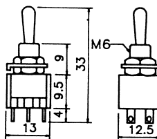
B068BW 3P MINIATURE TOGGLE SWITCH (SPDT) ON-ON 120V 5A (250V 2A)
