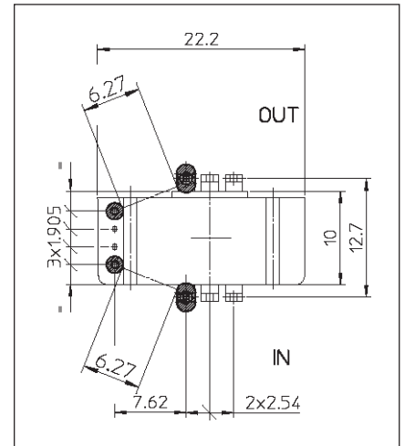
Fig. 19: Clearance distance
