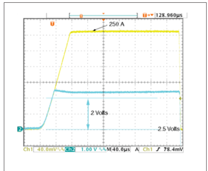
Fig. 5: Behaviour of the LTSR output during a positive overload of 10 \times I_n
