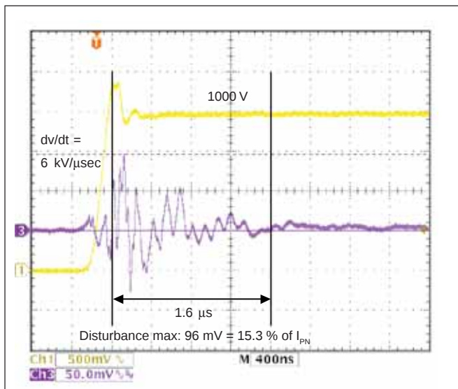
Fig. 3: Immunity to dV/dt variations of the LTSR (LTSR 25-NP)
