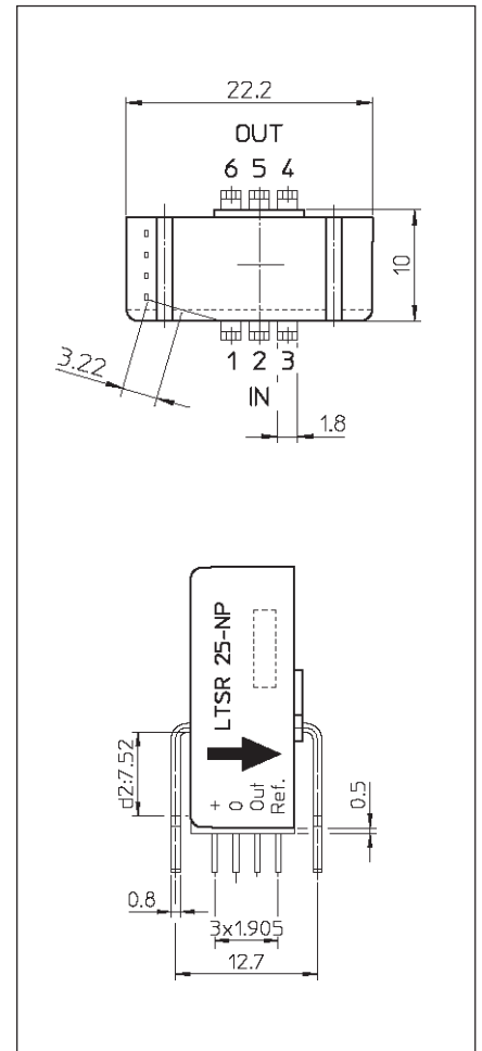
Fig. 20 + 21: Creepage distance
