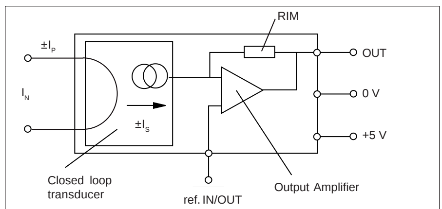
Fig. 6: LTSR 25-NP Operational principle
