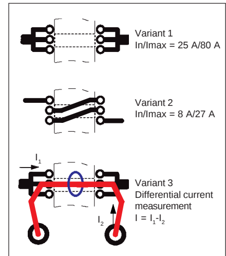
Fig. 18: The different possibilities for connecting the primary current circuit (e.g. LTSR 25-NP)
