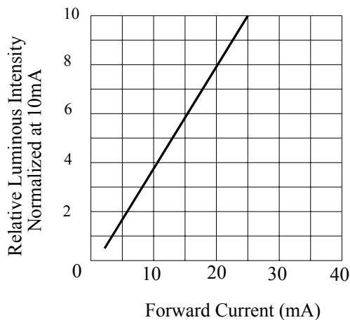
Fig.5 RELATIVE LUMINOUS INTENSITY
