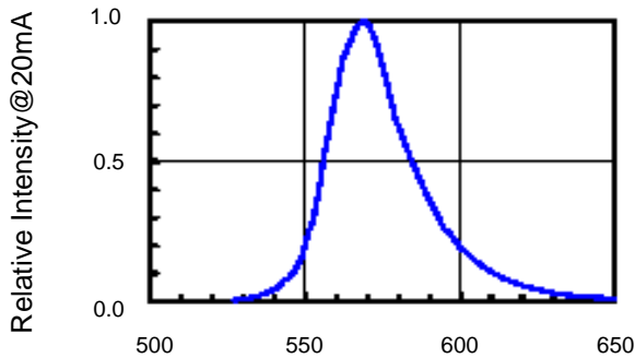
Wavelength (nm)
