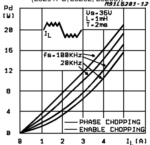
Figure 7b: Typical Power Dissipation vs I_L (L6201PS, L6202, L6203)
