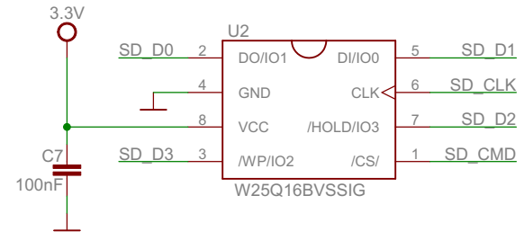
MOD-WIFI-ESP8266, board revision A
