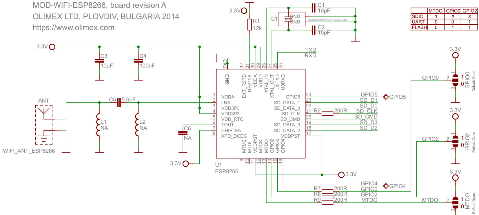
MOD-WIFI-ESP8266, board revision A
