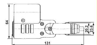
K3213 Auto plug to auto double jack (PBT) W/light ring W/fuse/10A CE
