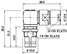
M579302 Right angle 1.6/5.6 female clamp type gold-pin (RG179U/3C2V)
