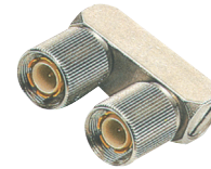
M579330 1.6/5.6 Female clamp type gold-pin (RG179U/3C2V)
