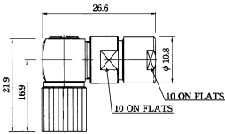
M579300 Right angle 1.6/5.6 male clamp type gold-pin (RG179U/3C2V)
