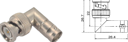
M5546 Right angle BNC male to BNC female gold-pin
