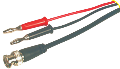
L41132 Test lead set banana plugs & BNC male L=3ft
