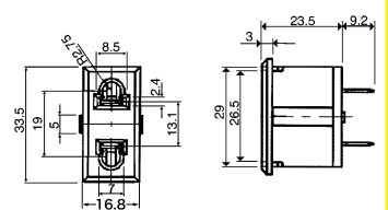
K25131 (K240A) Panel mount AC socket
