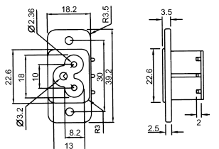
K2523 Panel mount AC socket
