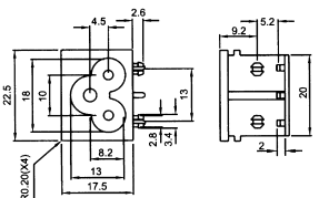
K2524 AC power socket 250V 16A
