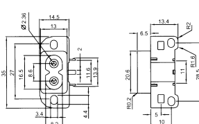
K25131 (K240A) Panel mount AC socket
