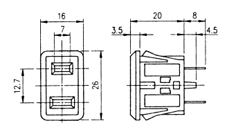
K2513 Panel mount AC socket (polarized)
