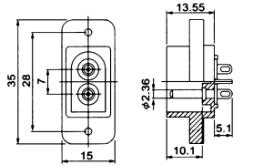
K250 Panel mount AC socket
