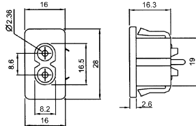
K2513 Panel mount AC socket (polarized)
