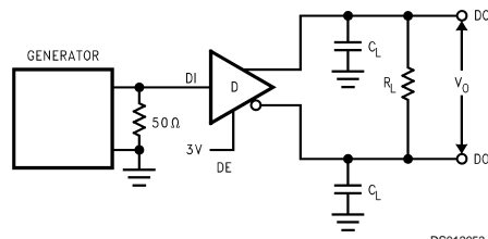
FIGURE 5. Driver Differential Propagation Delay Test Circuit
