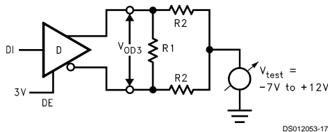
FIGURE 2. Driver V_{OD3}
