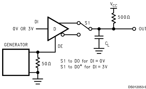
FIGURE 9. TRI-STATE and Sleep Mode Test Circuit ( t_{PZL} , t_{PSL} , t_{PLZ} )
