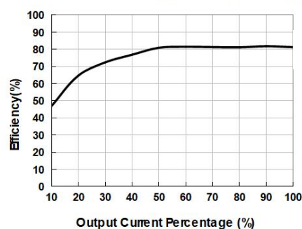
Efficiency Vs Output Load (Vin=24V)
