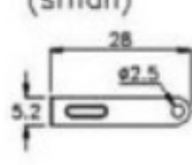
Metal Switch (small)
