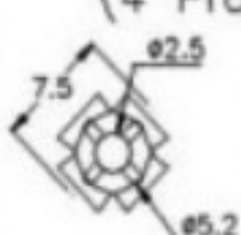
Female Contact (4 Prong)
