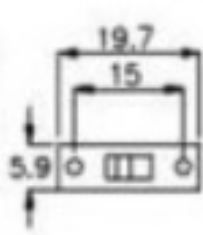
Switch
