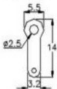
Female Contact (4 Prong)
