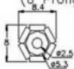
Female Contact (6 Prong)
