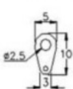
Small Contact
