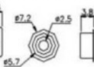
Male Contact
