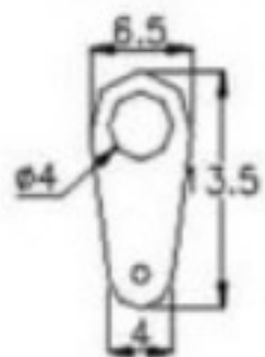
Female Contact (6 Prong)
