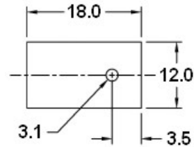
NYLON BUSH
