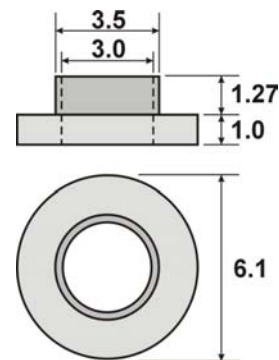
NYLON BUSH
