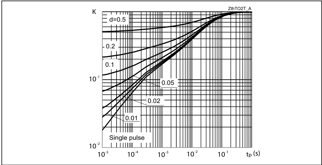
Figure 25. Thermal impedance
