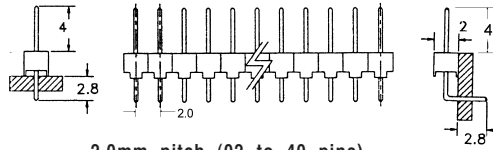
2.0mm pitch (02 to 40 pins)
