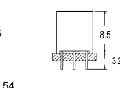
2.54mm pitch (09 to 96 pins)
