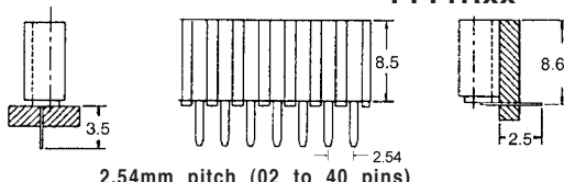
2.54mm pitch (02 to 40 pins)
