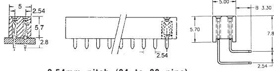
2.54mm pitch (04 to 80 pins)
