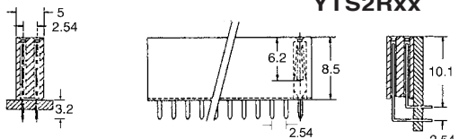
2.54mm pitch (04 to 80 pins)
