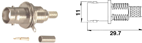
M558103 BNC FEMALE BULKHEAD CRIMP TYPE (RG58U/59U)
