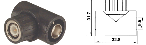
M558207 T-TYPE BNC MALE TO DOUBLE BNC FEMALE
