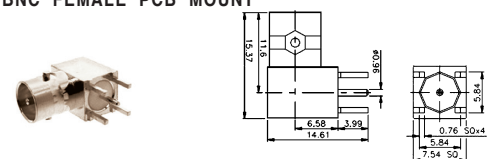
M558327 RIGHT ANGLE MINI BNC FEMALE BULKHEAD PCB MOUNT
