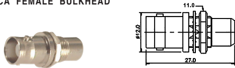
M558102 BNC FEMALE TO RCA FEMALE BULKHEAD
