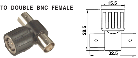
M558208 BNC MALE TO DOUBLE BNC FEMALE
