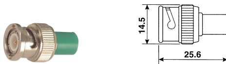
M558202 BNC MALE TERMINATOR 1/2W A:50 Ω B:75 Ω C:93 Ω
