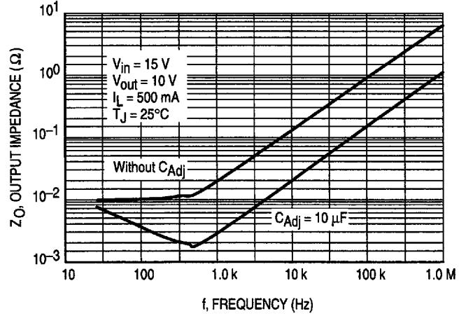
Figure 14. Output Impedance
