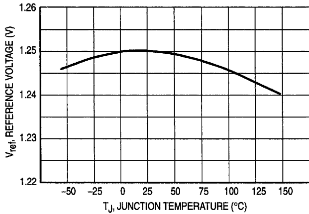
Figure 9. Temperature Stability
