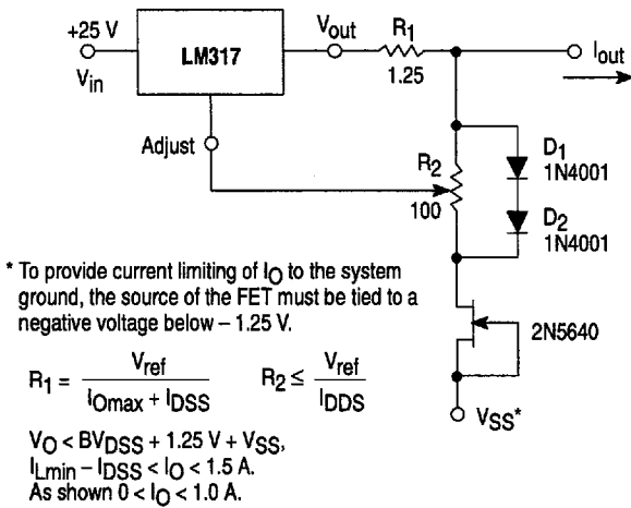
Figure 21. Adjustable Current Limiter
