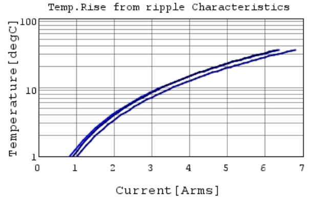
GRM31CD80J107MEA8 Temp.rise — 50kHz
