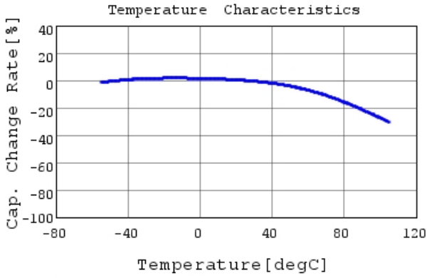
GRM31CD80J107MEA8 C-Temp. capchange, DC0.0V,
