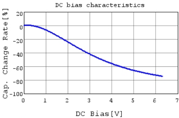
GRM31CD80J107MEA8 C-DC bias capchange, 25.0c
