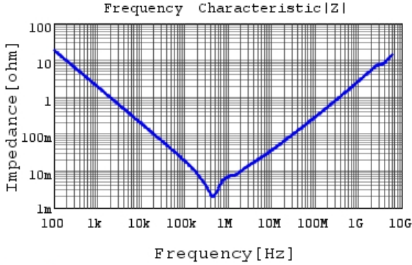
GRM31CD80J107MEA8 |Z| DCOV, 25degC
