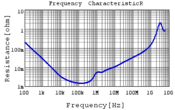
GRM31CD80J107MEA8 R DCOV, 25degC
