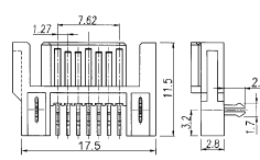
7P Serial ATA male SMD type YXSD07M
