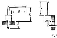
Pin header dual rows (right angle) YWRxx
