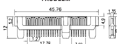
7+15P Serial ATA male DIP type YXSD22M
