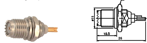
M55303 Mini UHF female bulkhead gold-pin
