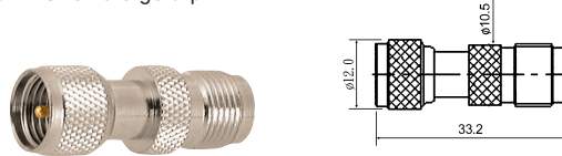
M55307 Mini UHF male to TNC female gold-pin
