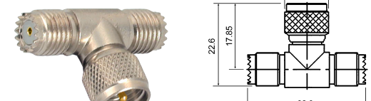
M55316 T-type mini UHF male to double female gold-pin
