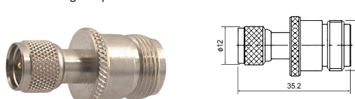
M55306 Mini UHF male to N female gold-pin
