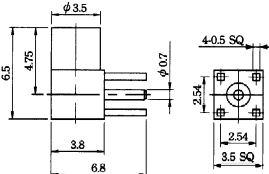
M52466 MMCX female solder type for semi-rigid cable (RG405U) (gold plated)
