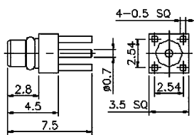
M52430 MMCX female bulkhead (gold plated)
