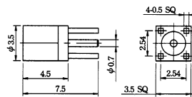
M52460 MMCX male solder type for semi-rigid cable (RG405U) (gold plated)
