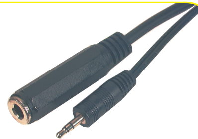
L448625 3.5mm Stereo plug to 6.3mm stereo jack L=0.2M
