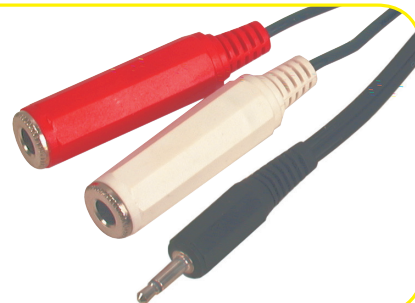
L448626 3.5mm Mono plug to 2 x 6.3mm mono jacks L=0.2M
