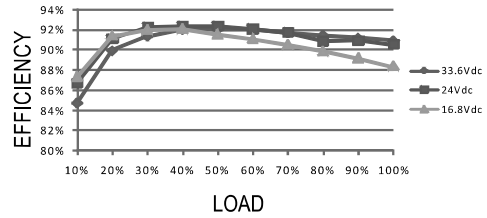
DDR-240B-48
