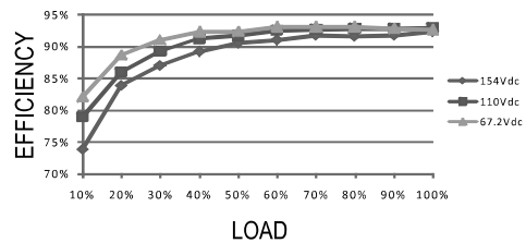
DDR-240D-48
