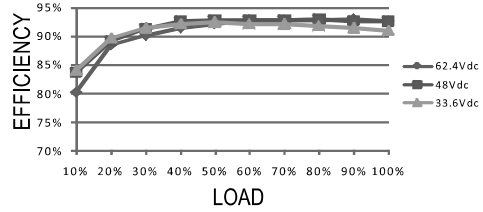
DDR-240C-48
