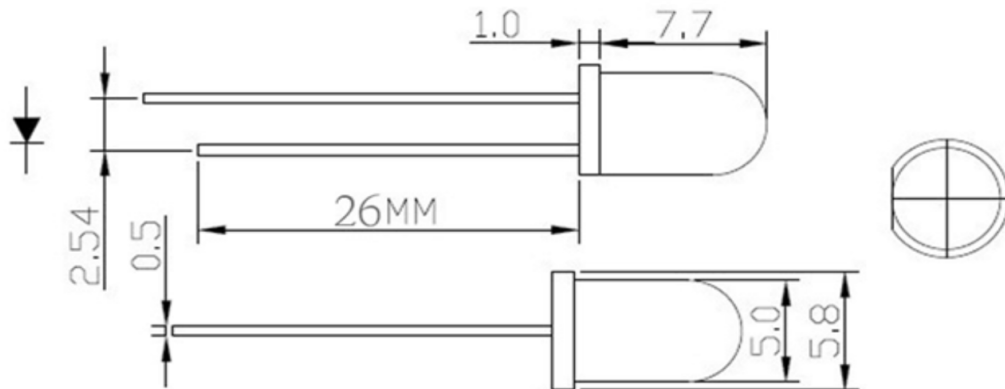
Product Drawing
