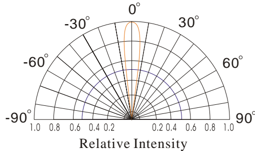
Beam Patter
