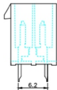
SECTIONAL DRAWING
