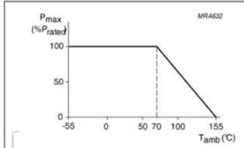
Fig. 7-1 Maximum dissipation (P) in percentage of rated power as a function of the operating ambient temperature (Tamb)
