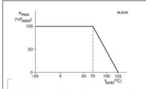
Fig. 7-2 Maximum dissipation (P) in percentage of rated power as a function of the operating ambient temperature (Tamb)
