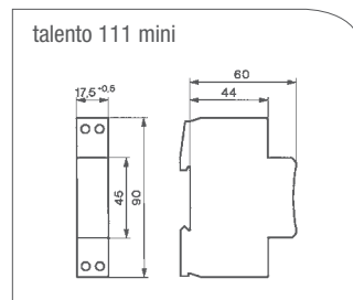
Dimensional drawings / circuit diagrams:
