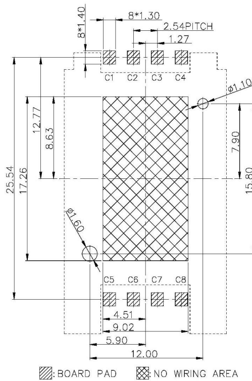
Unit: mm; Tolerances: ±0.05 mm Figure 5.4 Reference dimension for PCB layout (8 pins)
