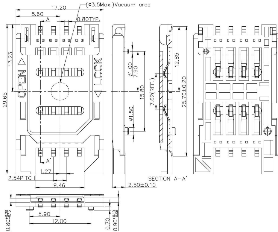
Unit: mm; Tolerances: ±0.15 mm Figure 5.3 Mechanical outline dimension (8 pins)
