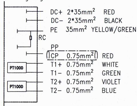
Wiring diagram
