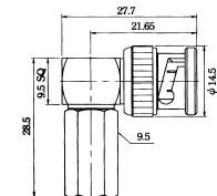
M55799 RIGHT ANGLE BNC MALE TWIST ON TYPE (RG58U/59U)
