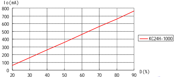
(Figure 6) Output current VS Pulse width of the PWM signal (f=200Hz)
