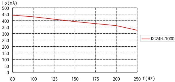
(Figure 5) PWM Frequency VS Output current(D=50%)
