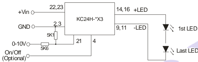
(Figure 7) Analogue dimming circuit
