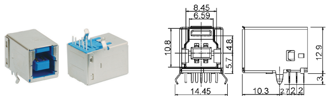
Y99012 USB 3.0 B type socket right angle
