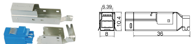
Y99016 USB 3.0 B type plug (molding type)
