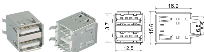
Y99005 USB A type dual socket
