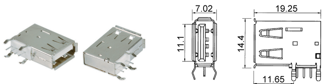
Y99002 USB A type socket upright
