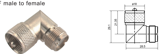
M5516 Right angle UHF male to female
