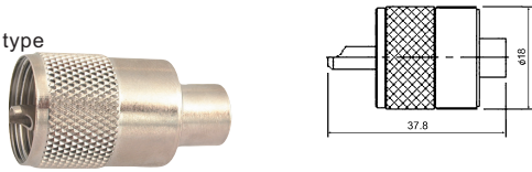
M5502 UHF male twist on type (RG8AU)
