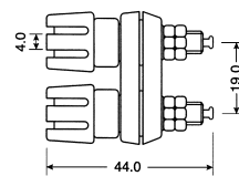
K2104 Double binding post (gold plated)
