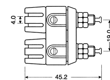
K2105 Double binding post (gold plated)
