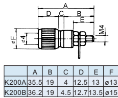
K2074 Binding post
