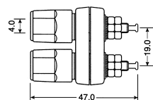
K2102 Double binding post
