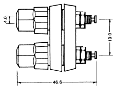
K2101 Binding post (gold plated)
