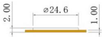
侧面图 Side View
