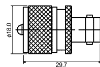
M5517 T-TYPE UHF MALE TO DOUBLE FEMALE
